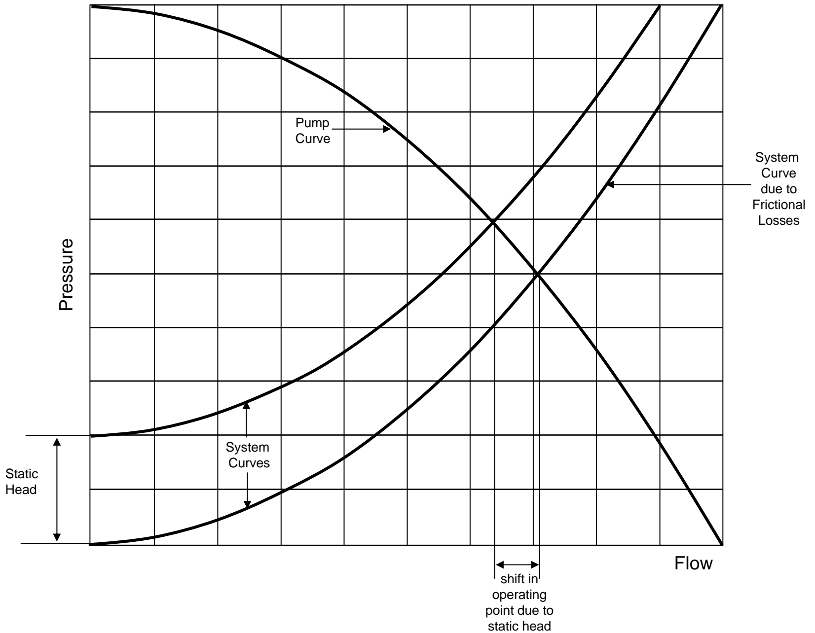
Figure 7-31b. Static Head Effect on Intersection of Pump Curve and System Curve
