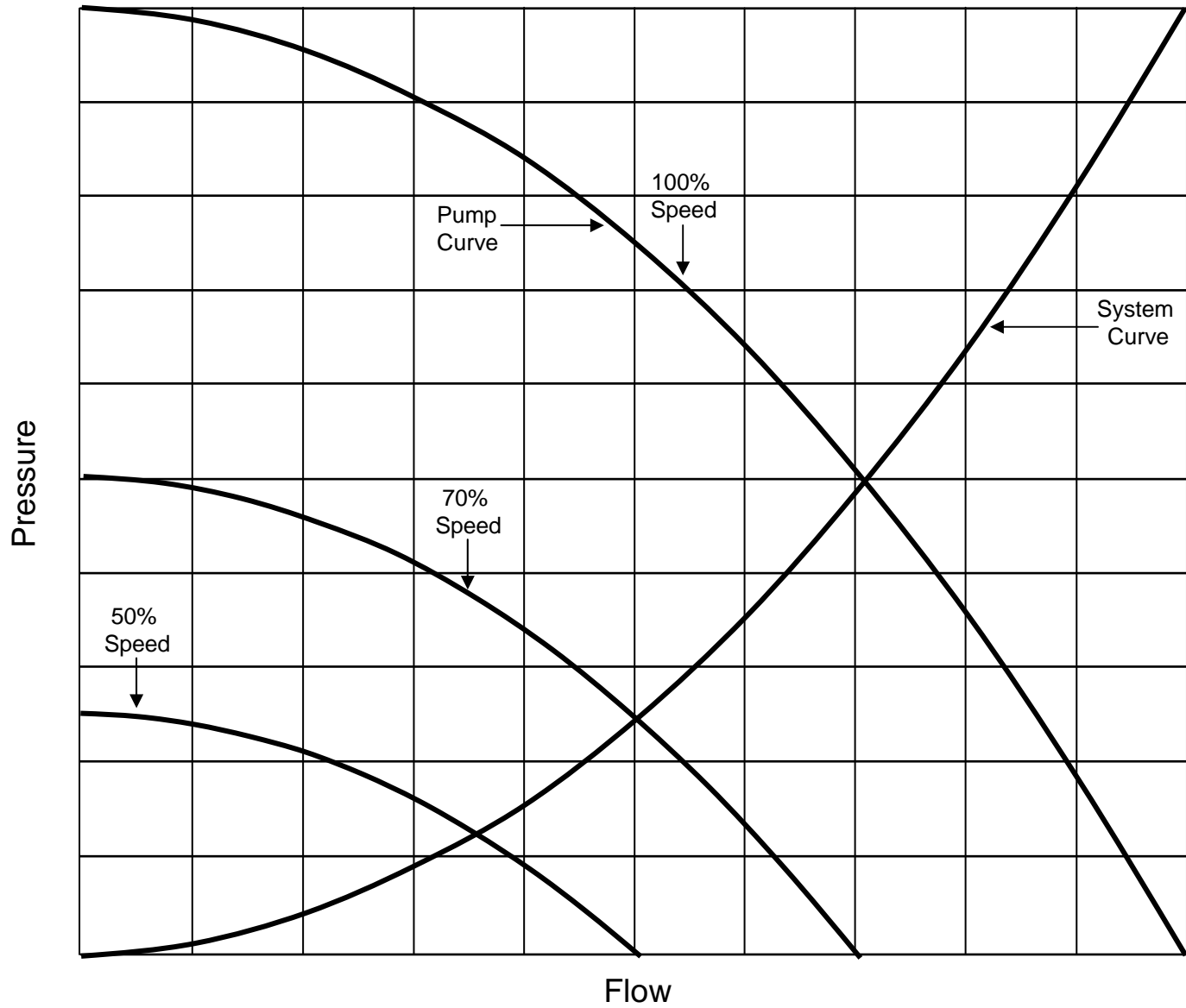
Figure 7-49a Pump and System Curves for VSD Flow Control (zero static head)
