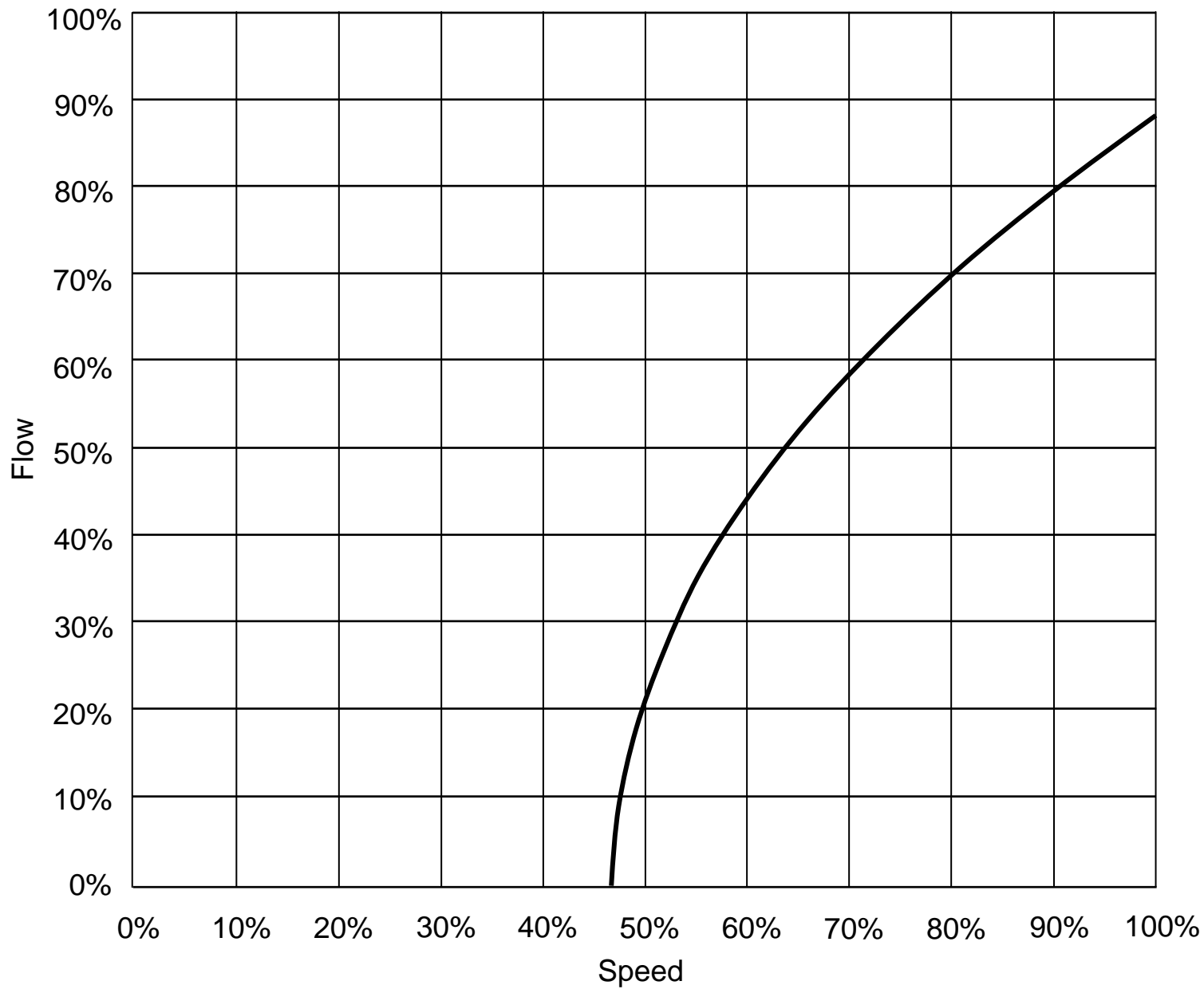
Figure 7-50b Effect of Static Head on VSD Flow Control
