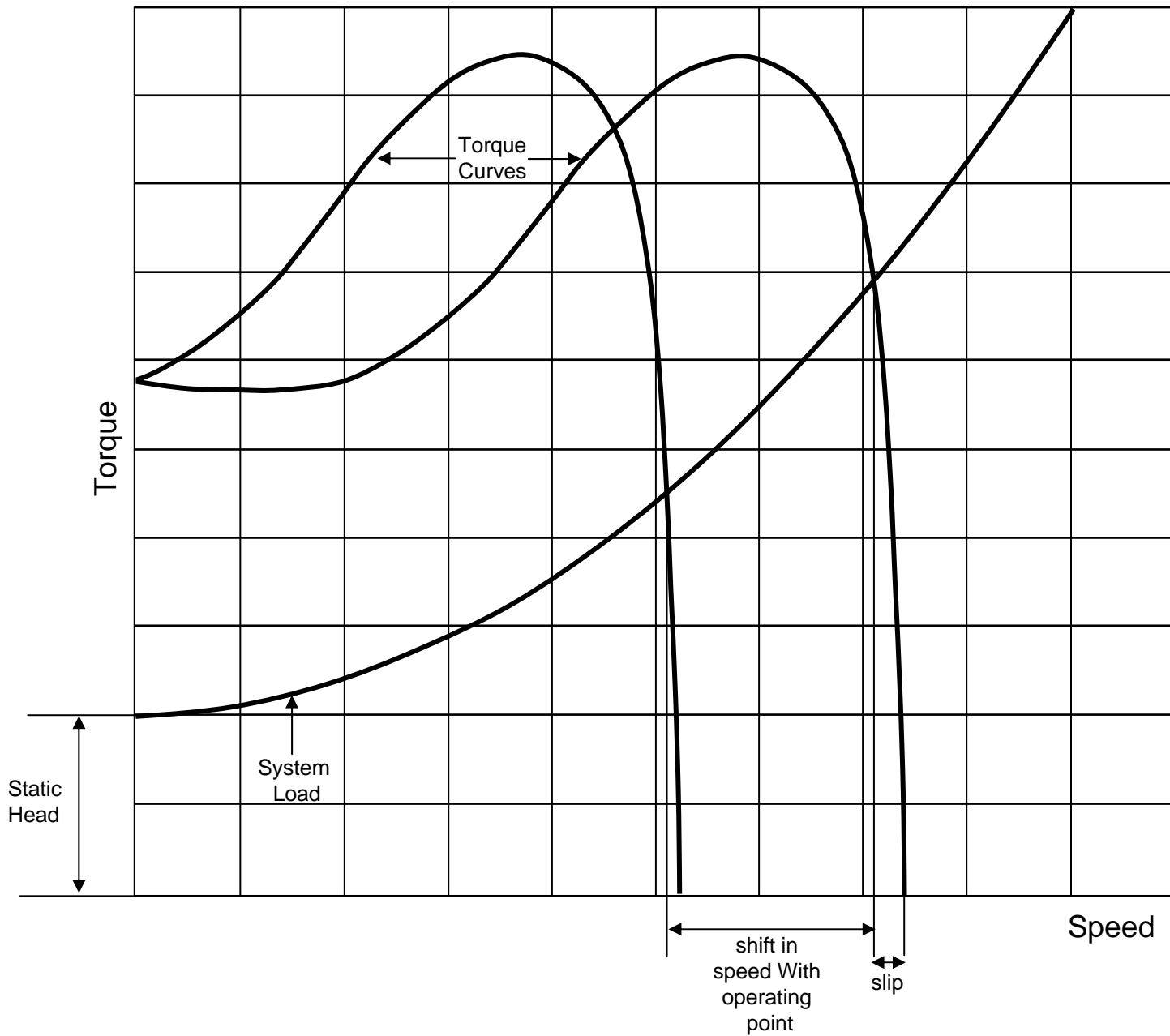
Figure 7-33. Shifting of Torque Curves by Torque and Current Control
