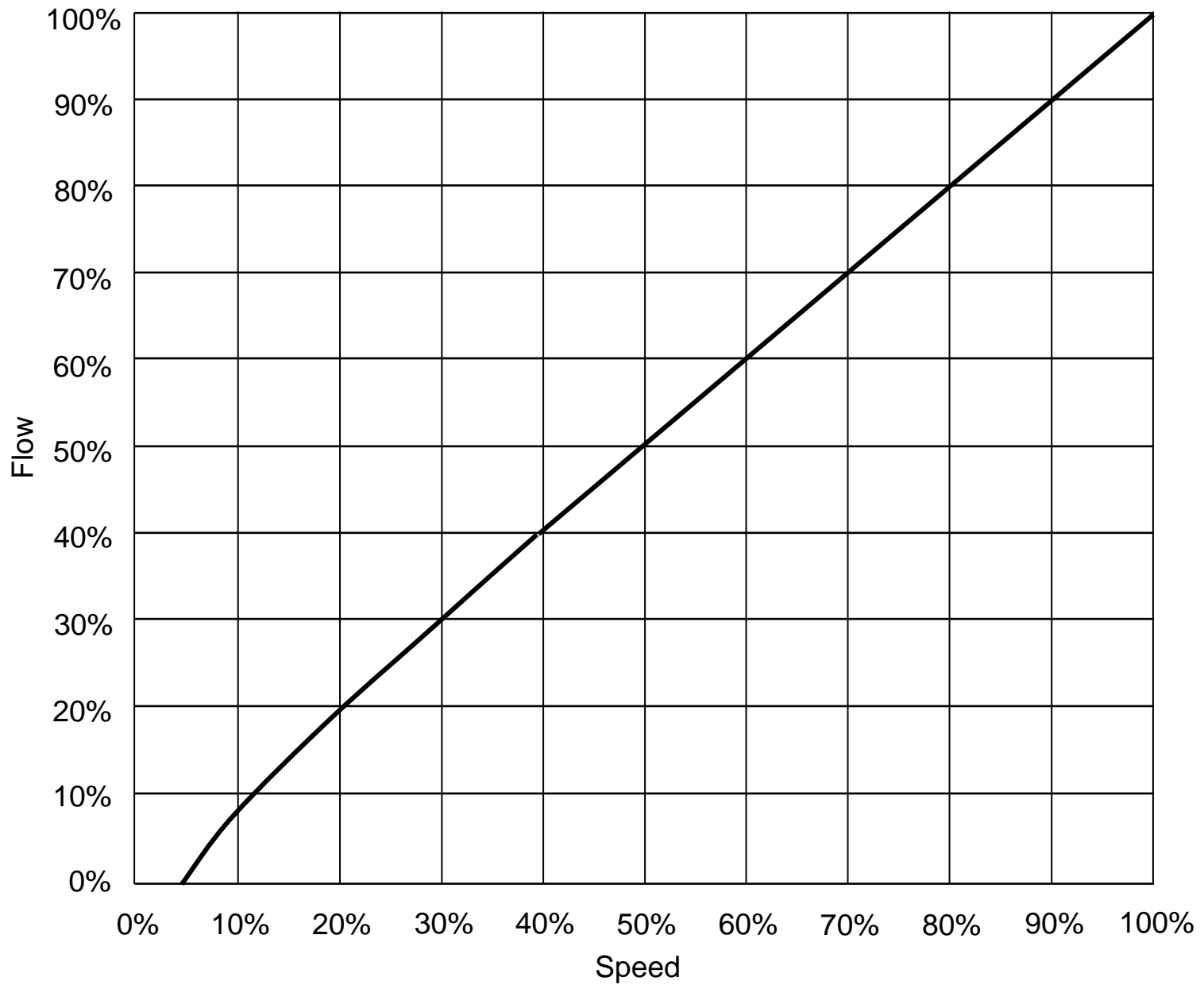
Figure 7-50a Effect of Pump Efficiency and Slip on VSD Flow Control
