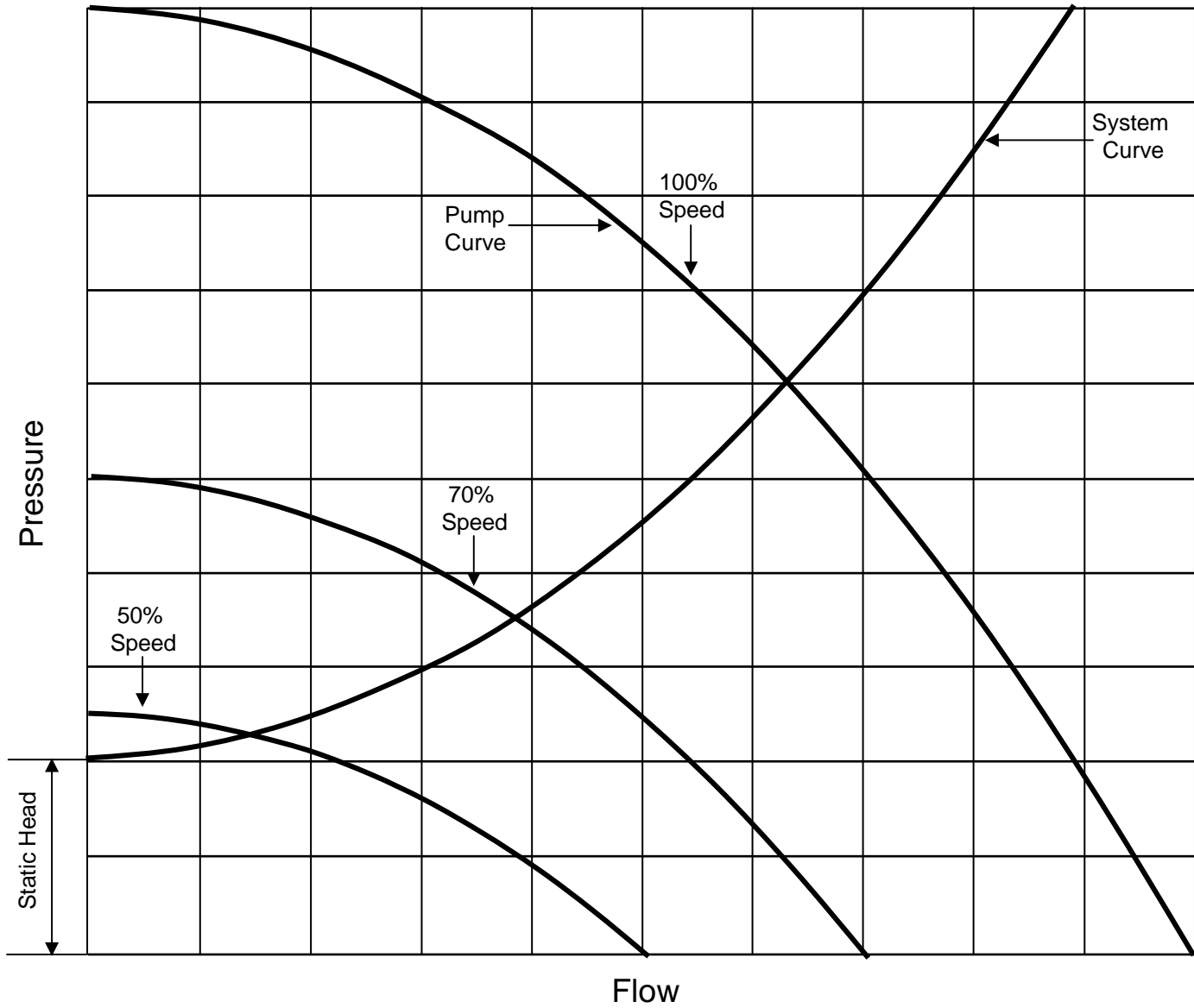
Figure 7-48b Pump and System Curves for VSD Flow Control (significant static head)
