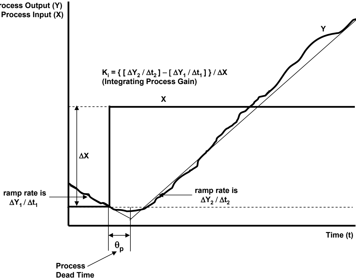
Integrating (Zero Feedback) Response
