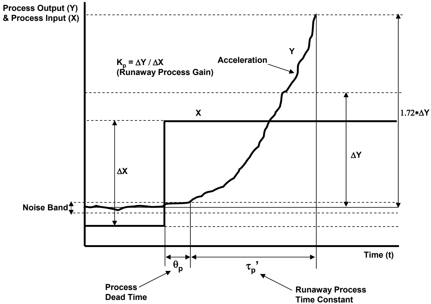
Runaway (Positive Feedback) Response
