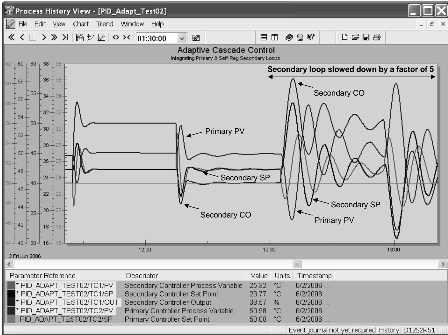
Interacting Oscillations in Cascade Loop from Slow Secondary Loop
