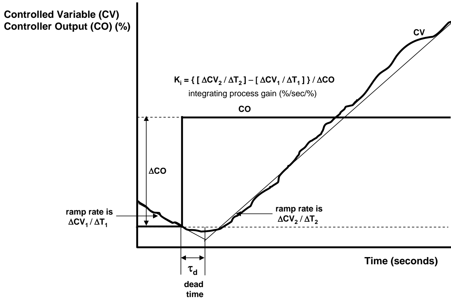
Open Loop Response of Integrating Process
