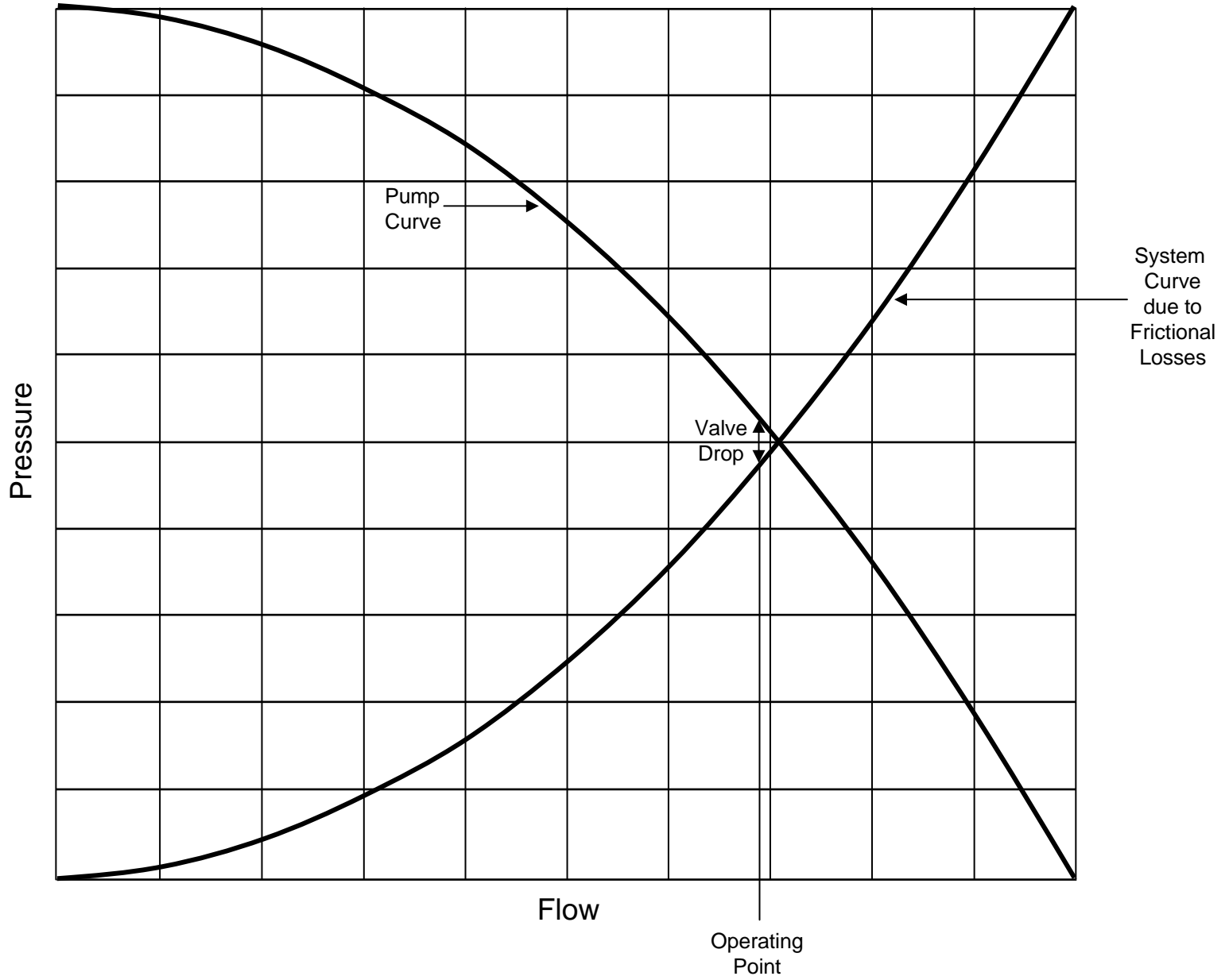
Figure 7-45. Available Valve Pressure Drop
