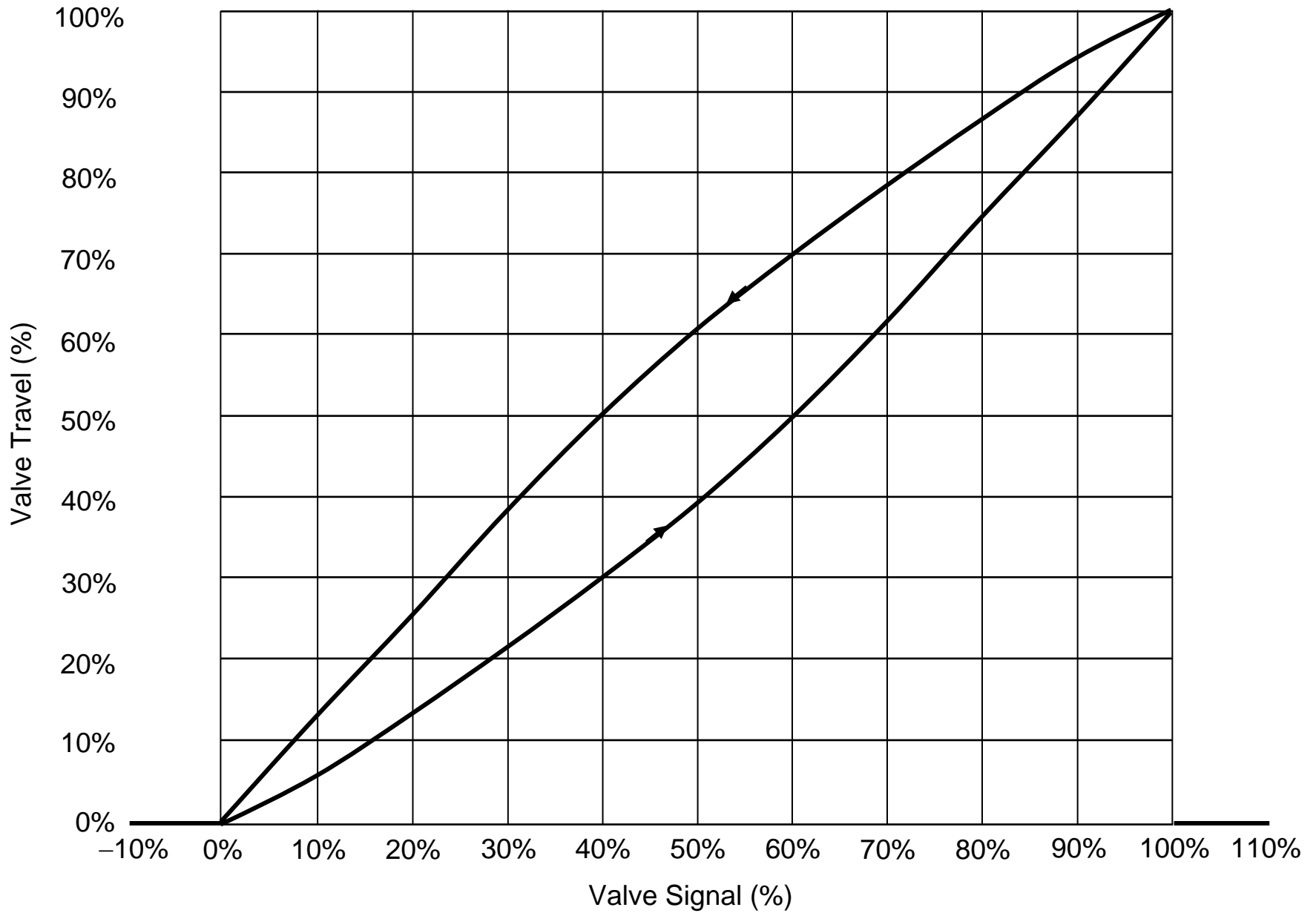
Figure 7-40a. Hysteresis from Energy Dissipation in Actuator (zero backlash and zero stick-slip)
