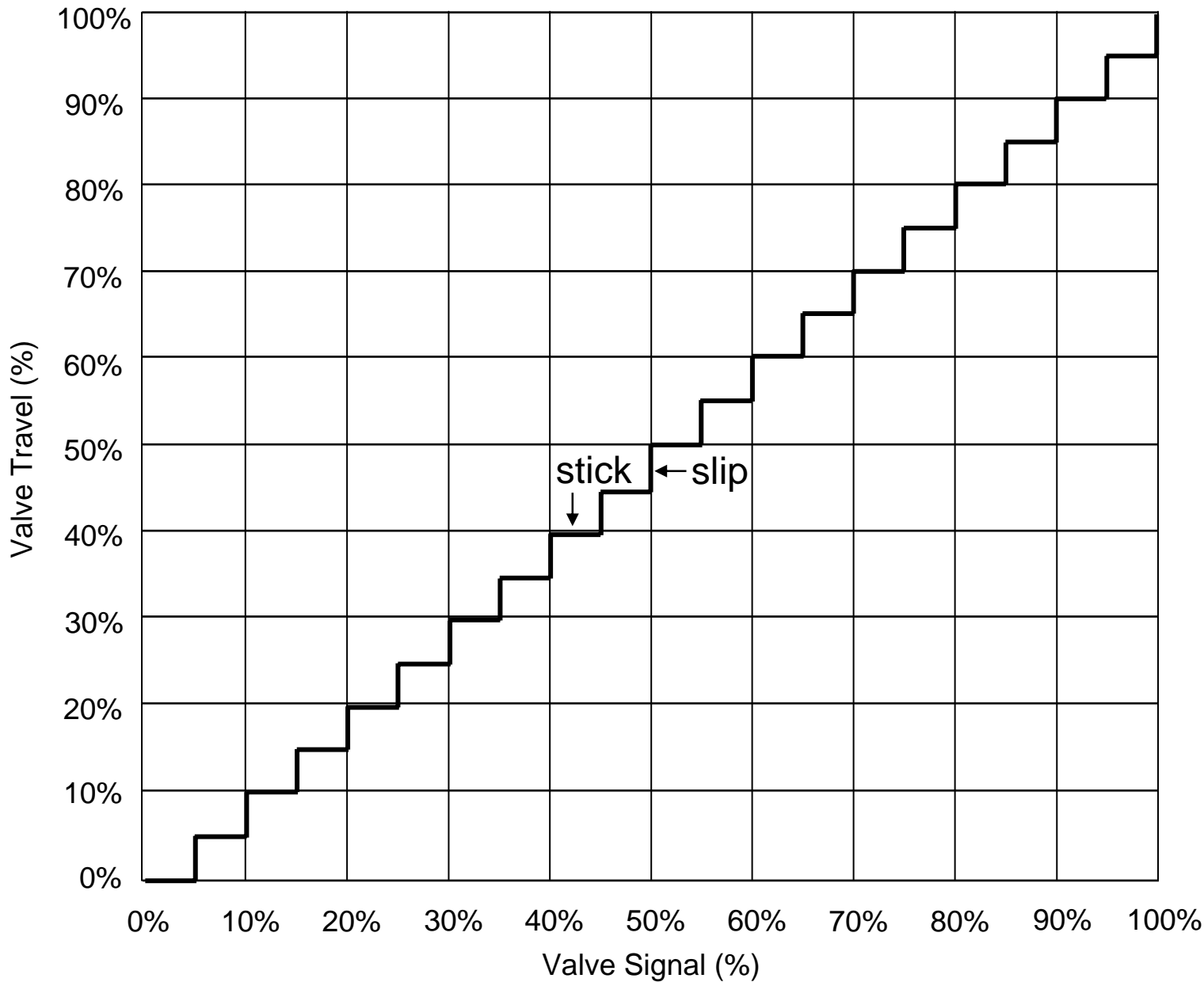
Figure 7-39. Resolution Limit from Stick-Slip (zero hysteresis and zero backlash )
