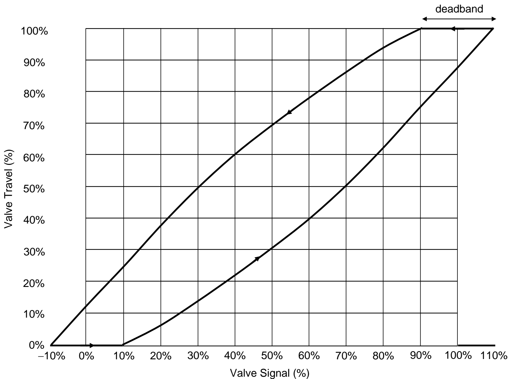
Figure 7-40b. Deadband from Backlash and Hysteresis from Energy Dissipation (zero stick-slip)
